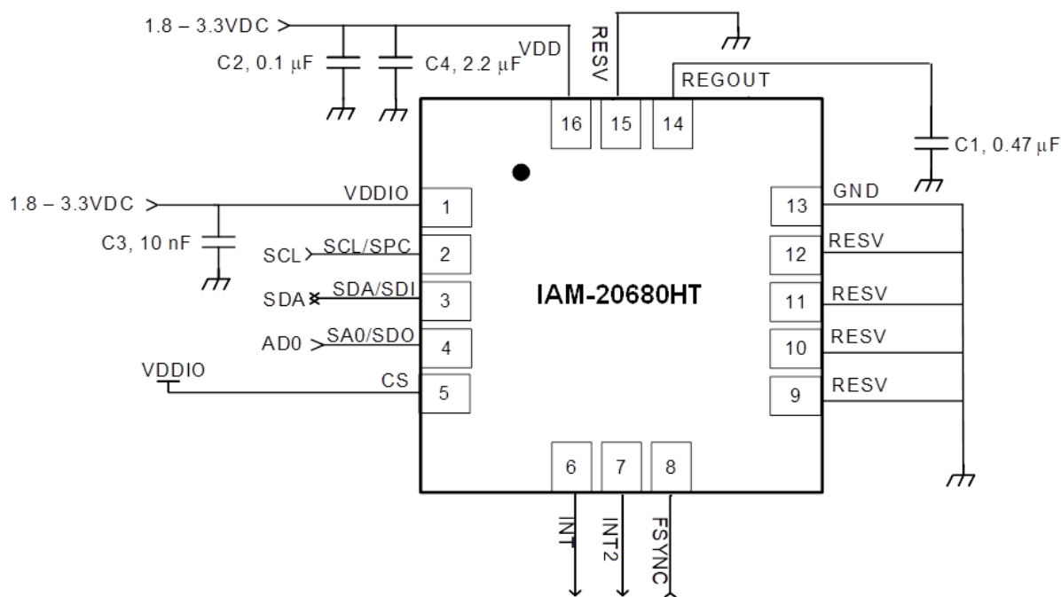
Figure 4. IAM-20680HT LGA Application Schematic
