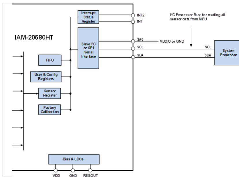
Figure 6. IAM-20680HT Solution Using I 2 C Interface
