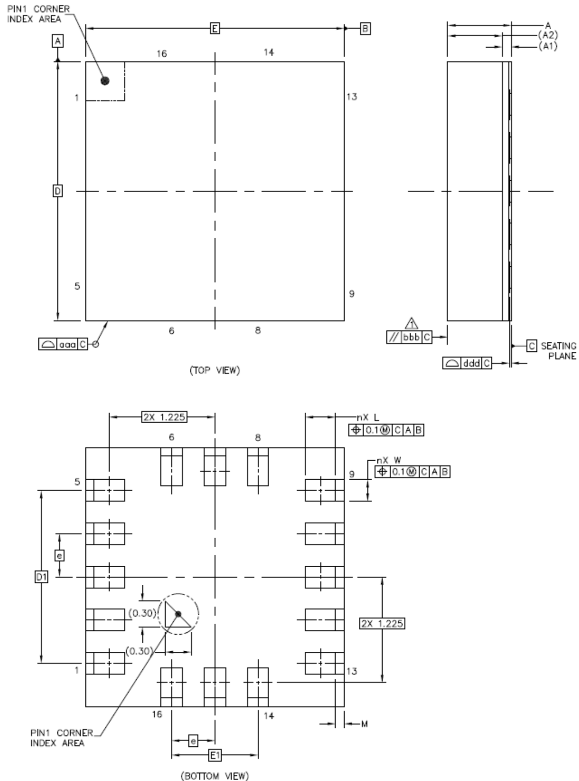
Figure 14. Package Dimensions
